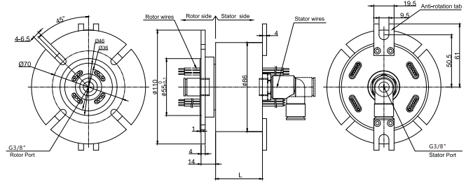
MAPH100-05 Dimensions
