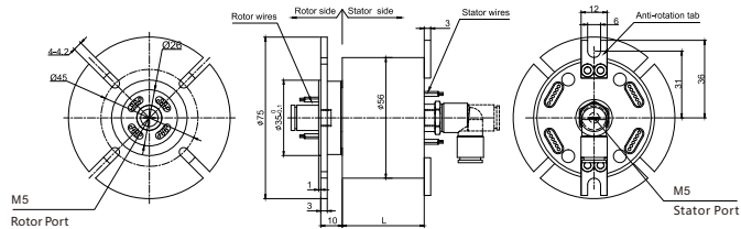
MAPH100-02 Dimensions
