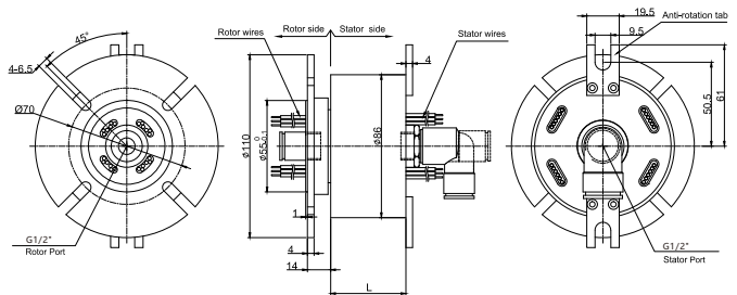
MAPH100-05 Dimensions
