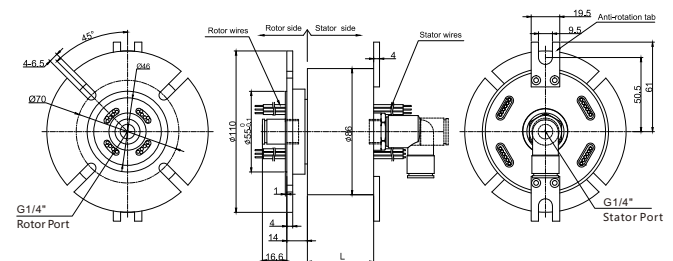
MAPH100-03 Dimensions
