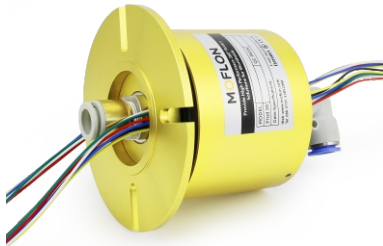
1 passage, G1/2
