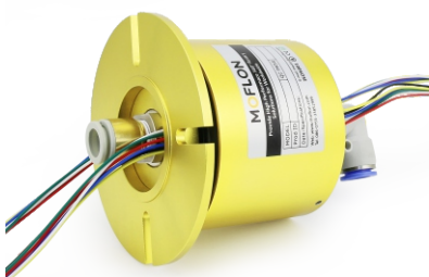
1 passage, G1/4
