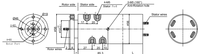
MAPH400-02 Dimensions
