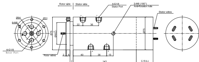
MAPH400-02 Integration of gas and electricity Dimensions
