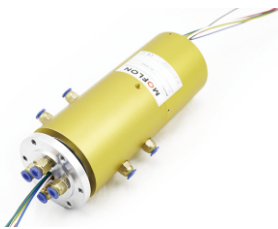
4 passages, G1/8
