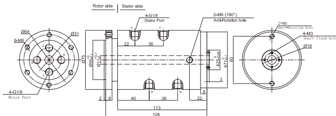
MAPH400-02 Integration of gas and electricity Dimensions
