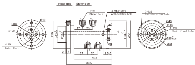
MAPH400-01 Integration of gas and electricity Dimensions
