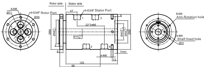
GJ4015-04 Size 4 ports in, 4 ports out, G3/8 Port
