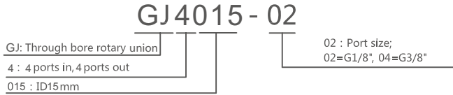
GJ4015-02 Size 4 ports in, 4 ports out, G1/8 Port
