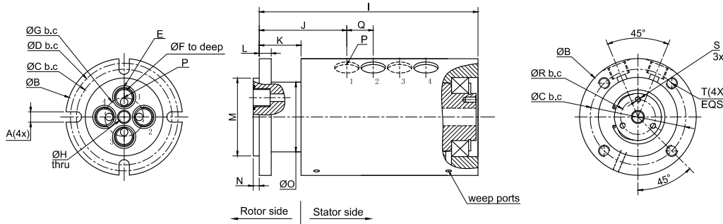
MGP4 Series (Multi-function Swivel) Dimensional Drawing
