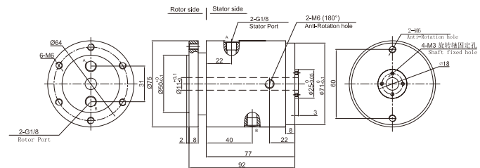
MAPH200-02Pneumatic/Hydraulic Slip Ring Dimensions
