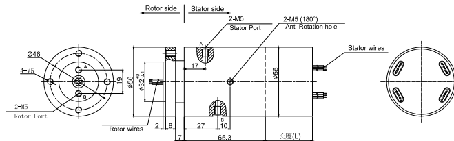
MAPH200-02 Dimensions
