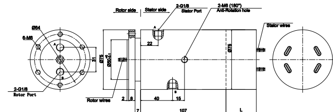
MAPH200-02Pneumatic/Hydraulic Slip Ring Dimensions
