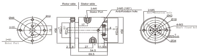
MAPH200-01Pneumatic/Hydraulic Slip Ring Dimensions
