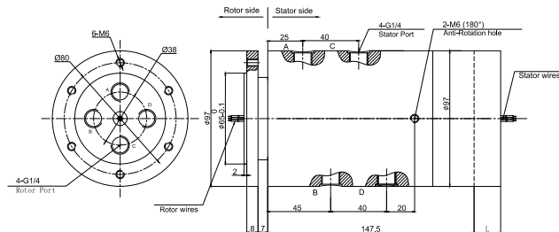
MAPH400S-03 Dimensions
