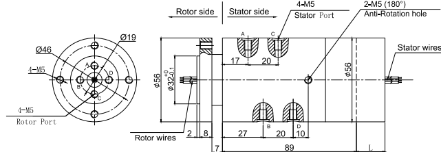
MAPH400S-02 Dimensions
