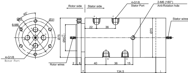
MAPH400S-03 Dimensions
