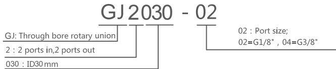
GJ2030-02 Size 2 ports in, 2 ports out, G1/8 Port
