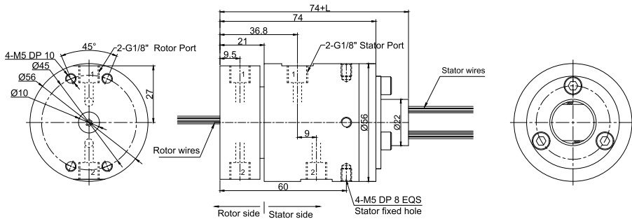
MK21S-S06(S12, S18, S24, S36) drawing 2 in 2 out, connection size G1/8"+06~36 wires x signal(2A)
