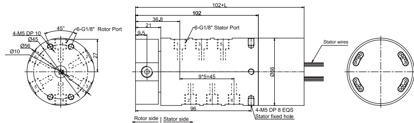
MK61-PXX-SXX drawing 6 in 6 out, connection size G1/8" + signal(5A)/10A
