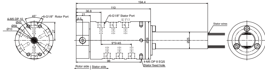
MK61S-S56 drawing 6 in 6 out, connection size G1/8"
