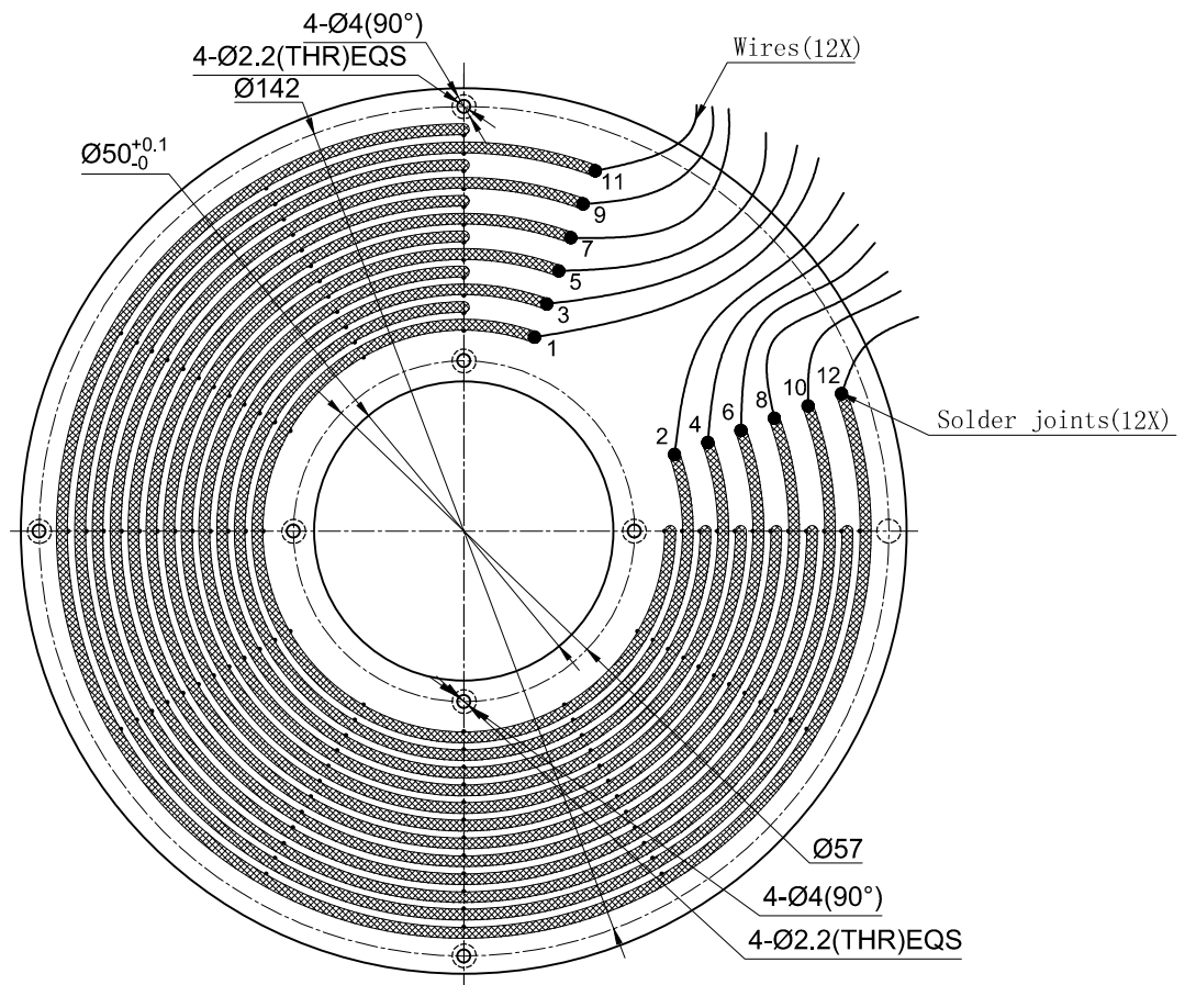
MPCB050-P1210
